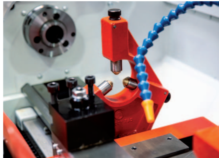
Steady rests. In addition to the tailstock, a wide range of steady rests is available for handling long workpieces. The picture shows a fixed steady rest.
