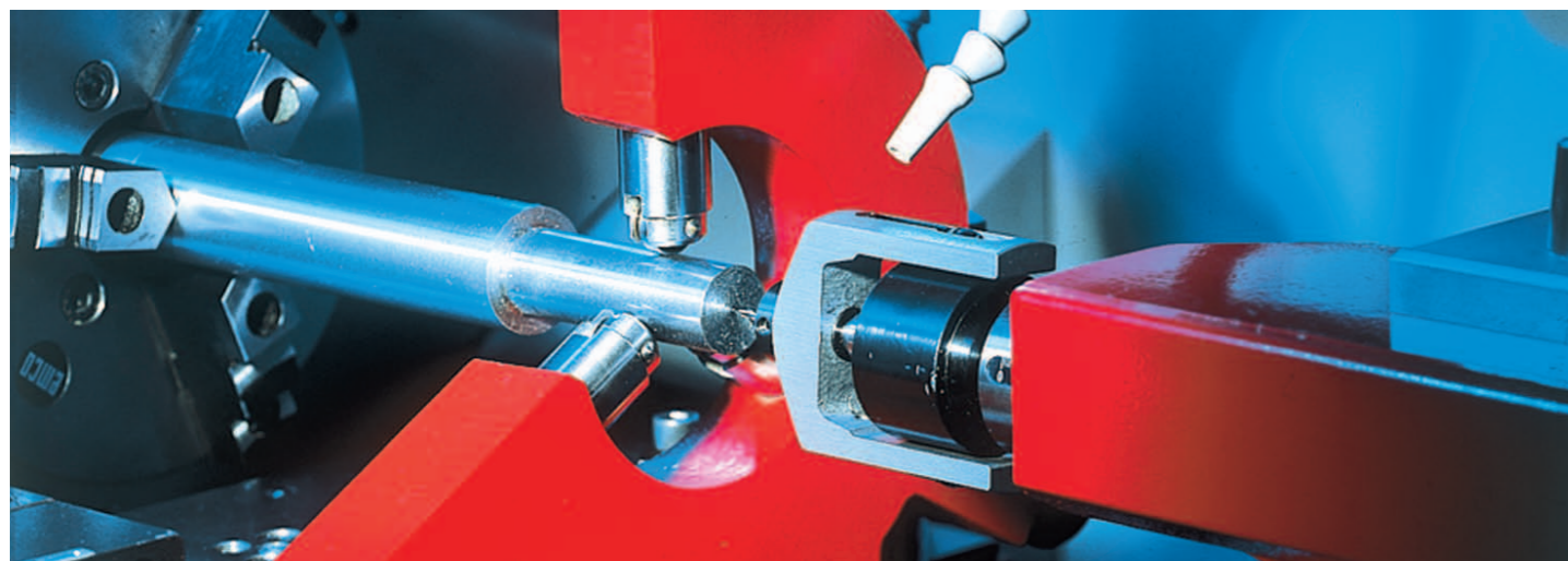
Machining with steady rest
