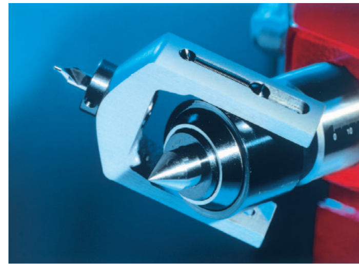
Center drill attachment for live centers
