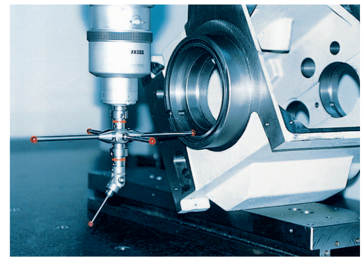
Headstock. Headstock quality is checked using a 3D Zeiss gauge. The main spindle's precision bearings can be adjusted. The diameter of the front bearing is 70 mm.
